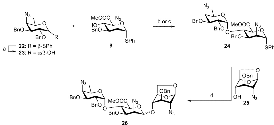
Scheme 2. Synthesis of protected trisaccharide 26 . Reagents and conditions: (a) NIS, TFA, DCM/H 2 O (10:1), 73%; (b) 22 , Ph 2 SO, Tf 2 O, TTBP, DCM, -60^{\circ}\text{C} then 9 , 55%; (c) 23 , Ph 2 SO, Tf 2 O, TTBP, DCM, -40^{\circ}\text{C} then 9 , 67%; (d) 25 , NIS, TMSOTf, DCM, 65% ( \alpha/\beta = 1:2).
