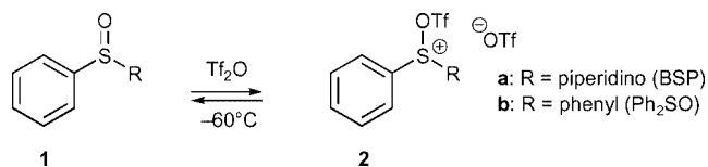
Figure 1. Sulfonium activator systems used for the activation of 1-thioglycosides.
